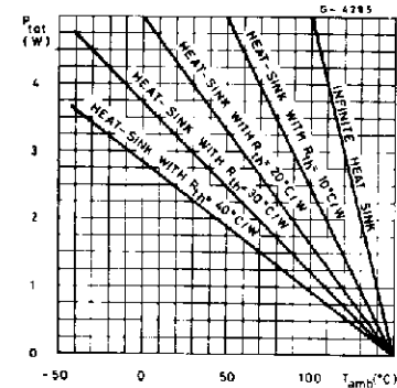
Figure 26. Maximum power dissipation vs. ambient temperature
